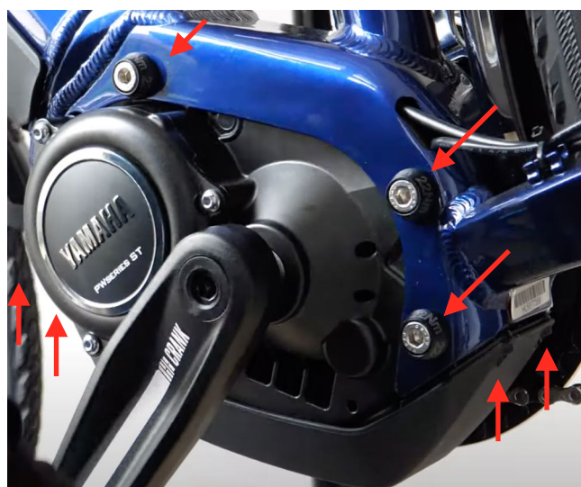
PW-ST motor
