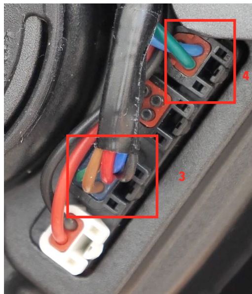
PW-S2 connectors
