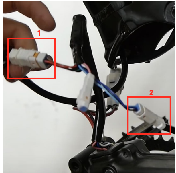
PW-X connectors
