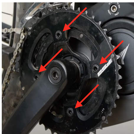
Remove chainrings
